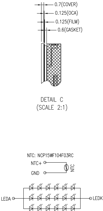
BACKLIGHT CIRCUIT DIAGRAM
