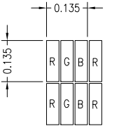
DETAIL A (SCALE 80:1)
